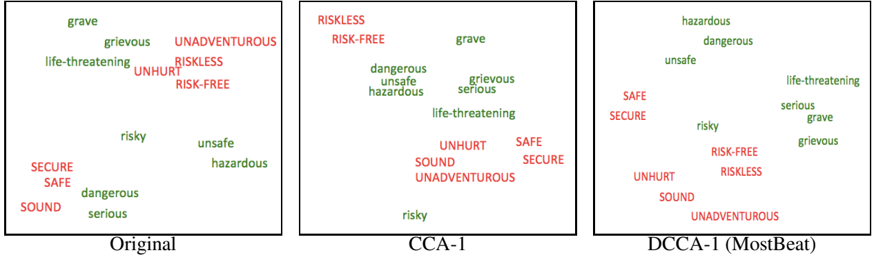
Figure 2: t-SNE visualization of synonyms (green) and antonyms (red, capitalized) of dangerous .
