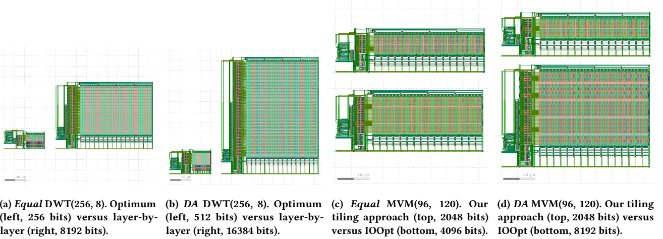
Figure 8: Physical layout comparison between power-of-two memory sizes among the different approaches described in Section 5.1 using the results in Table 1. DA refers to Double Accumulator.
