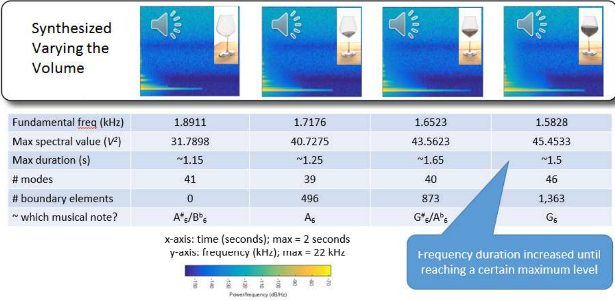
Figure 3.7: This figure displays the results of sound synthesis for our approach with liquid volume increasing from empty to glass half full; notice that the fundamental frequency decreases resulting in a lower pitch as the liquid increases
