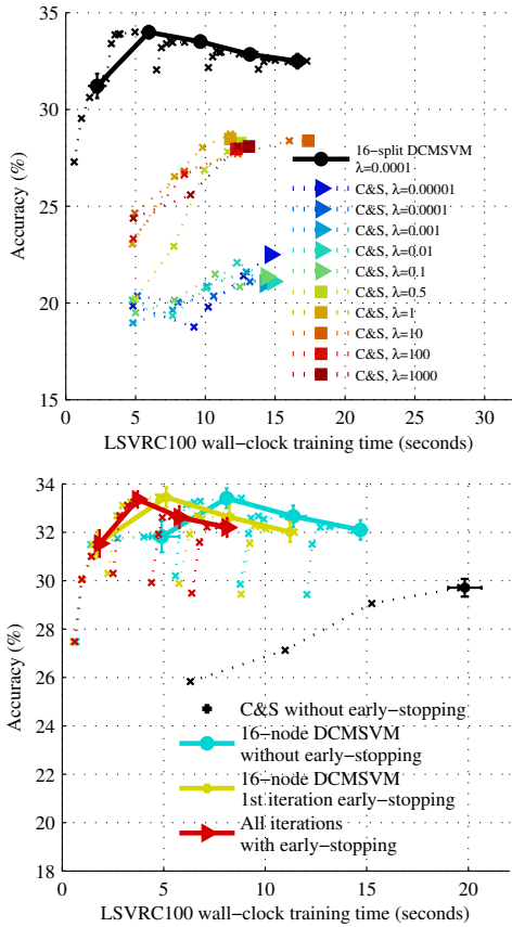
Figure 5. Comparison between our solution split across 16 nodes and Liblinear’s Cramer & Singer implementation on the ILSVRC100 data. Dashed lines indicate progress during optimization. Accuracy is measured on held out data. Error bars indicate variation in time and accuracy across different train/test splits. Top Shows that no \lambda allows a single split to match 16 splits in generalization accuracy, see Sec. 4.1. Bottom Effects of early stopping over 6 validation splits ( \lambda = 10 ) see Sec. 4.3.
